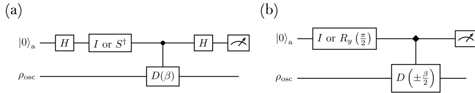
Figure 1.1: Figure: circuit diagram for tomography.
