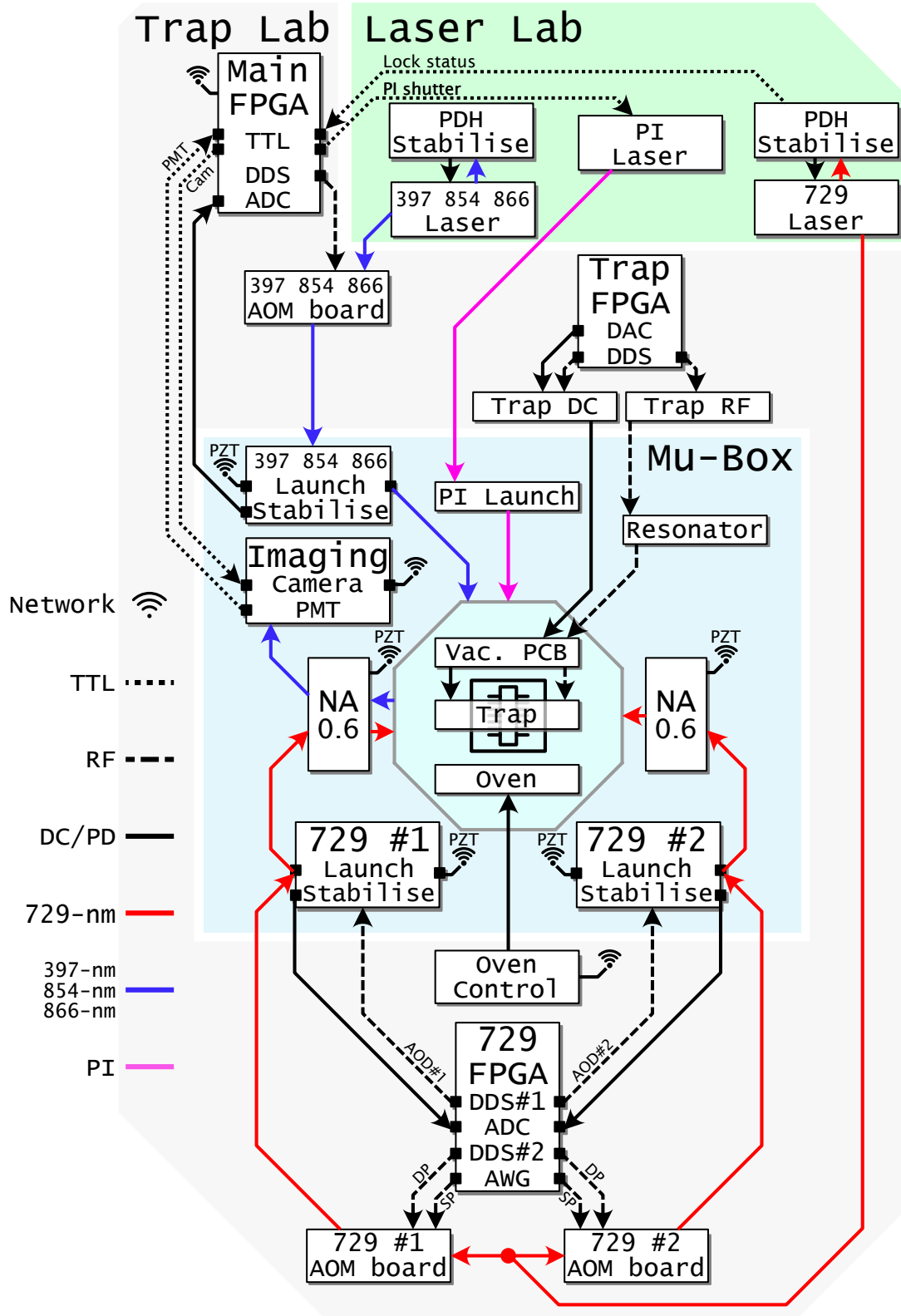
Figure 1.1: Block diagram schematic of the FastGates apparatus. Blocks resemble discrete subsystems, which shall be discussed within this chapter. Lines resemble relevant optical (free-space or in-fibre), RF, DC, and communication paths between subsystems. Block location signifies whether the device is in-vacuum, within the magnetic shielded (MuMetal) box, within the “trap-lab”, or within the “laser-lab”.
