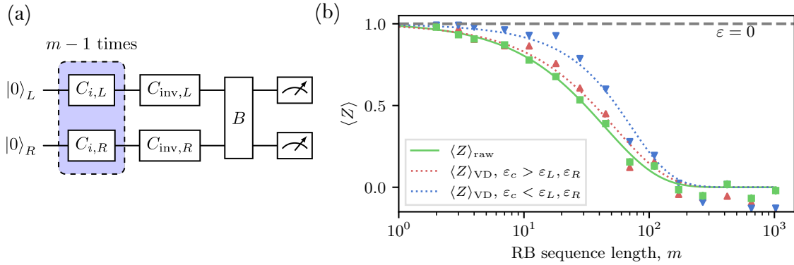
Figure 1.8: Figure: Cicruit diagram of RB + VD, exp data for noise floor for two copy B-matrix, with and without spatial correlations
