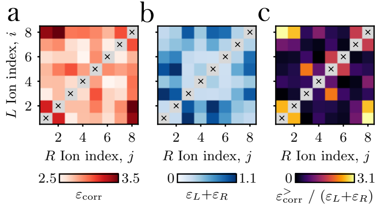
Figure 1.15: Correlated and local error per Clifford measured for all qubit pairs after applying k -copy RB to an 8 ion chain. Noise is dominated by position dependent duration of R_x(\pi/2) gates consistent with inhomogeneous illumination by the global drive. Panel (a) displays the extracted correlated errors, \epsilon_{\text{corr}}^{(i,j)} for each qubit pair, (i, j) . Panel (b) displays the sum of both independent depolarising errors, (\epsilon_L + \epsilon_R)^{(i,j)} . Panel (c) displays the ratio of excess correlated noise (offset from phase noise injection), (\epsilon_{\text{corr}}^{>})^{(i,j)} = \epsilon_{\text{corr}}^{(i,j)} - \epsilon_{\text{corr}}^{(0)} to the sum of local errors given in (b). This plot highlights the outer qubits are dominated by spatially correlated errors.
