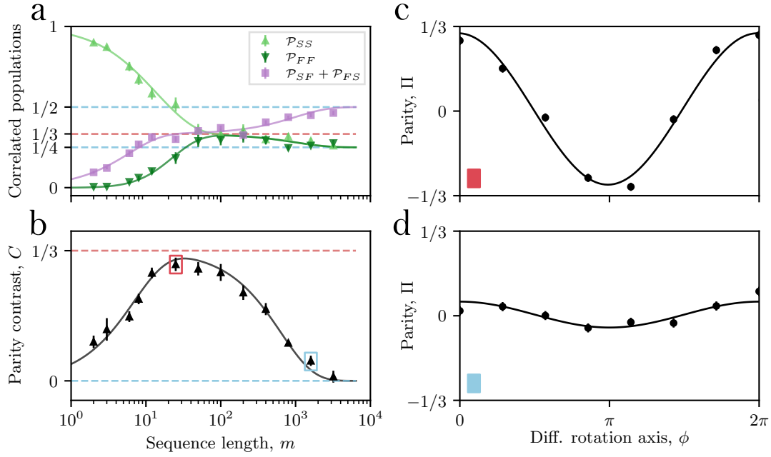
Figure 1.9: Parity contrast versus sequence length; (a) shows the standard Z measured correlated populations. (b) shows parity contrast — a signal proportional to occupation of the symmetric-trace sector. Solid lines are multi-exponential decays given by Eq. 1.29 and Eq. 1.43 for (a) and (b) respectively. Dashed lines indicate the expected asymptotes. (c) and (d) show example parity fringes for sequences of m = 25 and m = 1600 Clifford gates respectively.
