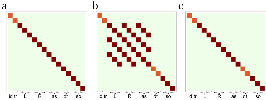
Figure A.1: Liouville operator representation of error channels after twirling over Cl_1^{\otimes 2} , ordered by the irrep basis (Schur basis). (a) Common noise , (b) Continuous ZZ , (c) Stochastic ZZ . Orange blocks represent an entry of 1, green represent 0, and red represent a decay with dependence on m .
