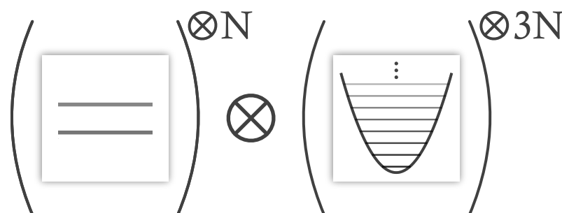
Figure 2.1: A schematic representation of the hybrid qubit-qumode register in the trapped-ion system. A system of N physical ions, with qubits encoded in the electronic levels and qumodes in the secular motion of the ion chain, provides N qubits and 3N qumodes.
