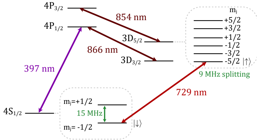
Figure 2.2: Electronic energy levels of ^{40}\text{Ca}^+ — the ion species used in this thesis. The levels are split by the Zeeman effect due to a \approx 5\text{ G} external magnetic field (splitting shown explicitly for the |4S_{1/2}\rangle and |3D_{5/2}\rangle manifolds). The transition wavelengths required for cooling and control over the ion are highlighted. The chosen qubit levels are labelled by |\downarrow\rangle , |\uparrow\rangle .
