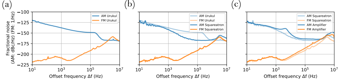
Figure 3.3: Characterisation of the RF chain. (a) SSB spectra for AM and FM, given as fractional noise, measured after the Urukul . (b) Measured after the Squareatron . (c) Measured after the amplifier.
