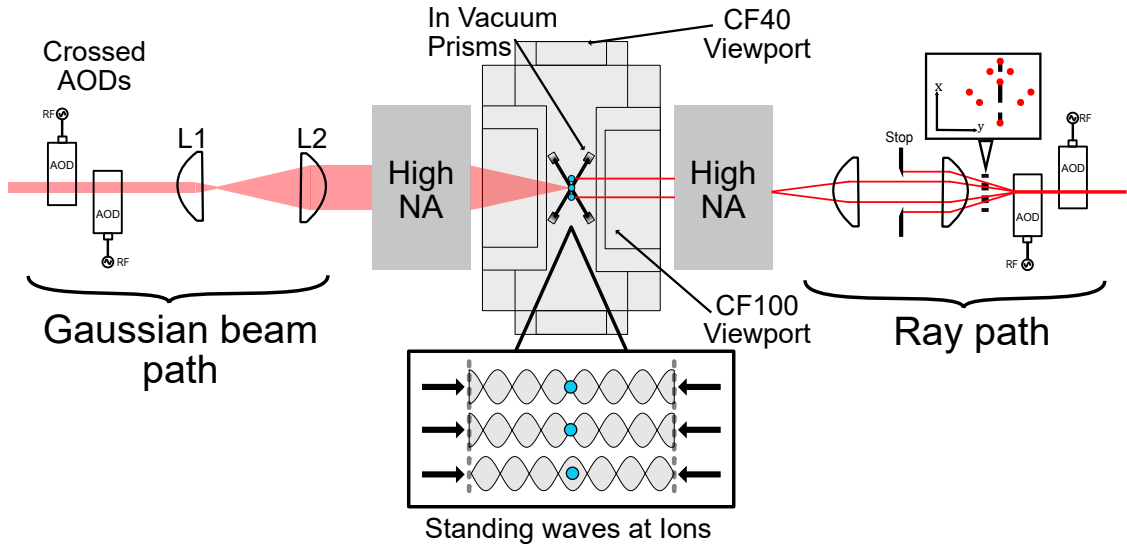
Figure 2.4: The standing wave single addressing system. Dual high NA objectives focus the light to a tight waist at the ions location. AODs are used to steer the light to only selected ions. The left hand side of the figure shows the Gaussian profile of the light, whilst the right hand side shows a ray representation of how two singly addressing spots are formed at the ions. L1 is a telecentric scanning lens and in combination with L2 form a beam expander.
