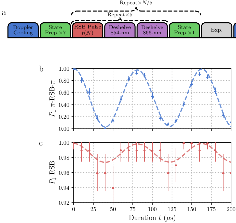
Figure 3.8: a) Example pulse sequence for one experimental shot including pulsed sideband cooling. The Exp. block represents an arbitrary sequence of operations, for the experiment under study, such as a thermometry sequence. The blue blocks represent Doppler cooling and readout (section 3.2.2), the green blocks represent qubit state preparation (section 3.2.1), the red blocks are RSB pulses with varying durations t(N) , and the purple blocks are deshelling pulses. After every 5 sideband cooling pulses, there is an interleaved state preparation sequence to ensure there is no population trapped outside of the closed cooling cycle. The RSB length is linearly increased with pulse number N , upto the expected RSB R(\pi) -pulse duration for n = 1 . b, c) Thermometry scans after Doppler and sideband cooling. The red points are the populations measured via on-resonance RSB pulses, and the blue points are the populations after a sequence of R(\pi) -RSB- R(\pi) with varying RSB probe durations. The dashed lines are fits to a thermal Fock state distribution, with truncation at n = 100 . The extracted mean occupation number is \bar{n} = 0.03(1) , and \eta\Omega/(2\pi) = 11.6(1) kHz.
