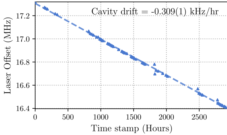
Figure 2.6: Cavity drift over 125 days measured by reference to the ion transition. The laser offset here is with respect to running all 729-nm AOMs at their central frequencies. Outliers are due to bad fits of the ion transition frequency, not due to changes in the cavity resonance.
