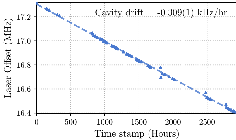
Figure 3.11: Cavity drift over 125 days measured by reference to the ion transition. The laser offset here is with respect to running all 729-nm AOMs at their central frequencies. Outliers are due to bad fits of the ion transition frequency, not due to changes in the cavity resonance.
