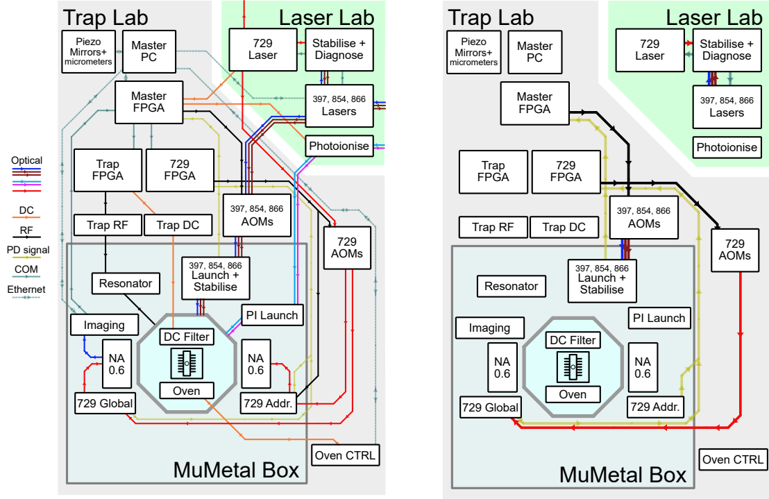
Figure 3.1: Block diagram schematic of the FastGates apparatus. Blocks resemble discrete subsystems, which shall be discussed within this chapter. lines resemble relevant optical (free-space or in-fibre), RF, DC, and communication paths between subsystems. The right panel highlights closed feedback loops for laser power and frequency stabilisation. Block location signifies whether the device is in-vacuo, within the magnetic shielded (MuMetal) box, within the “trap-lab”, or within the “laser-lab”.
