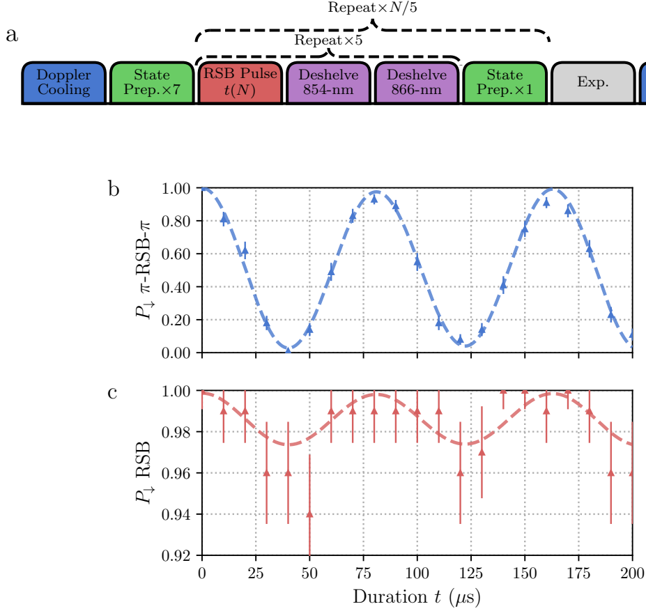
Figure 4.8: a) Example pulse sequence for one experimental shot including pulsed sideband cooling. The Exp. block represents an arbitrary sequence of operations, for the experiment under study, such as a thermometry sequence. The blue blocks represent Doppler cooling and readout (section 4.2.2), the green blocks represent qubit state preparation (section 4.2.1), the red blocks are RSB pulses with varying durations t(N) , and the purple blocks are deshelling pulses. After every 5 sideband cooling pulses, there is an interleaved state preparation sequence to ensure there is no population trapped outside of the closed cooling cycle. The RSB length is linearly increased with pulse number N , upto the expected RSB R(\pi) -pulse duration for n = 1 . b, c) Thermometry scans after Doppler and sideband cooling. The red points are the populations measured via on-resonance RSB pulses, and the blue points are the populations after a sequence of R(\pi) -RSB- R(\pi) with varying RSB probe durations. The dashed lines are fits to a thermal Fock state distribution, with truncation at n = 100 . The extracted mean occupation number is \bar{n} = 0.03(1) , and \eta\Omega/(2\pi) = 11.6(1) kHz.
