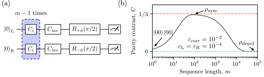
Figure 1.4: Probing coherence of the mixed state after k-copy RB. Panel (a) shows a circuit that first twirls the state over Cl_1^{\otimes 2} , and then applies differential \pi/2 -pulses with variable phase, \phi , to recover parity oscillations. Panel (b) shows the expected contrast of the oscillations as a function of sequence length when both local depolarising and common noise is present. The dashed lines indicate expected asymptotes for depolarising (blue) and for common noise (red).
