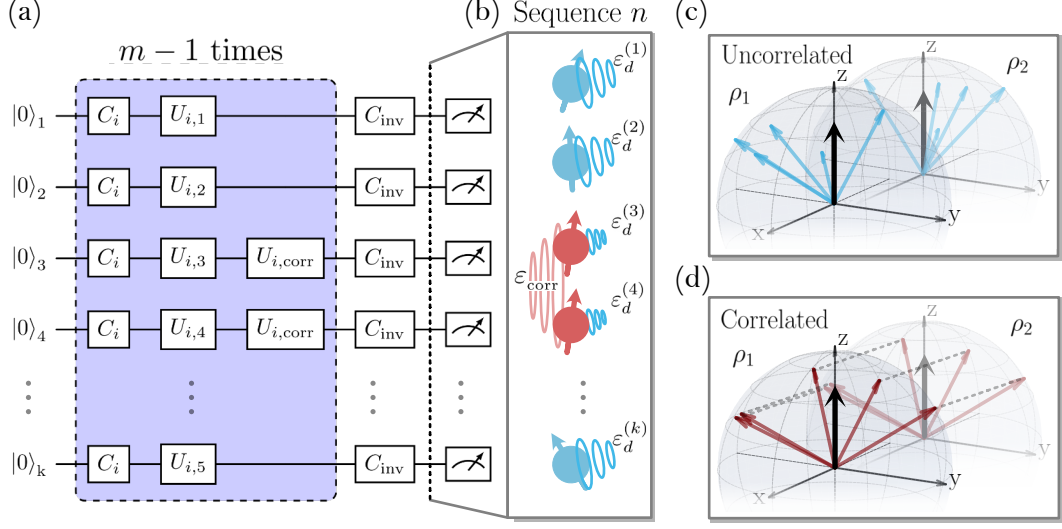
Figure 1.3: k -copy RB applies identical single-qubit Clifford sequences in parallel to all qubits. (a) shows the circuit diagram for a single RB random sequence. (b-d) illustrate the distinction between uncorrelated and common noise (a type of correlated noise) in the final-state trajectories.
