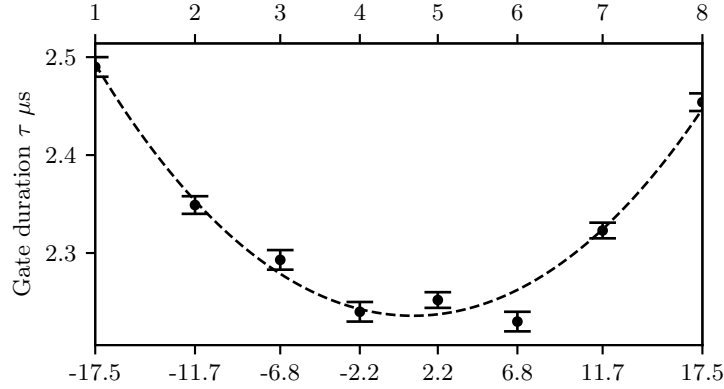
Figure 1.12: Missing x axis labels Variation of \pi -pulse gate duration along eight ion chain due to global beam Gaussian profile.
