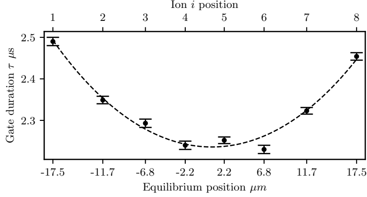
Figure 1.12: Variation of \pi -pulse gate duration along eight ion chain due to global beam Gaussian profile.
