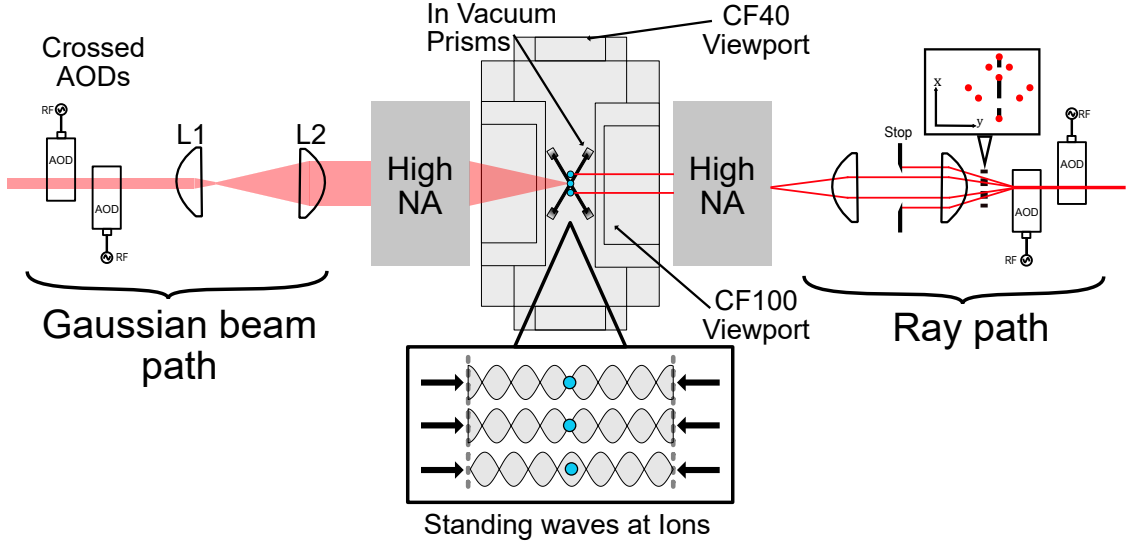
Figure 2.6: The standing wave single addressing system. Dual high NA objectives focus the light to a tight waist at the ions location. AODs are used to steer the light to only selected ions. The left hand side of the figure shows the Gaussian profile of the light, whilst the right hand side shows a ray representation of how two singly addressing spots are formed at the ions. L1 is a telecentric scanning lens and in combination with L2 form a beam expander.
