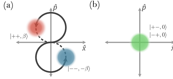
Figure 2.6: Phase space motion with spin-conditioning for MS gate, also with walsh modulation.
