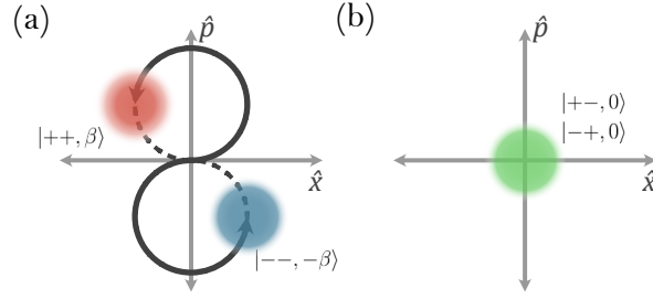
Figure 2.6: Phase space motion with spin-conditioning for MS gate, also with walsh modulation.
