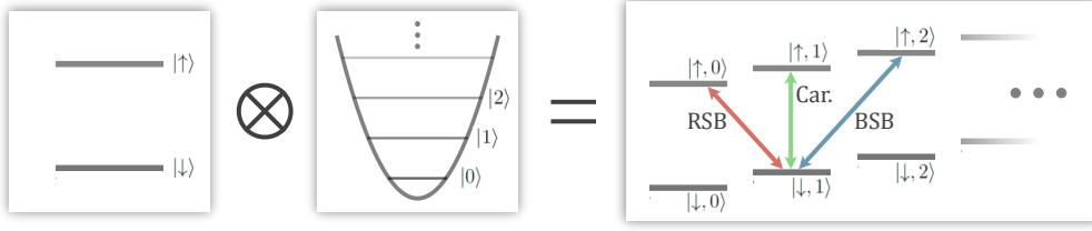
Figure 2.5: JC and AJC applied to |\downarrow, 1\rangle
