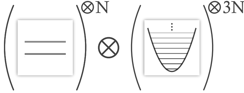
Figure 2.1: Spin otimes motion
