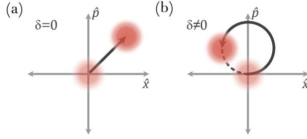
Figure 2.4: Phase space motion
