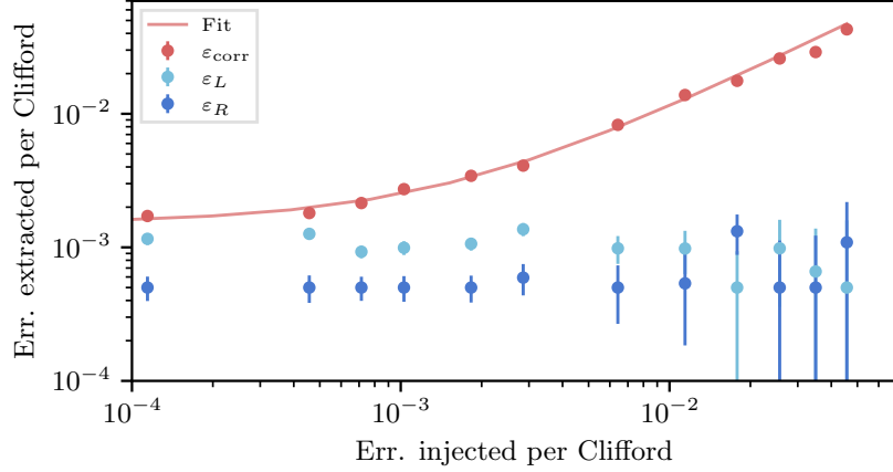
Figure 5.9: Injecting correlated noise between two qubits via common drive phase noise. Points correspond to fitted error per Clifford from full k-copy RB experiments. The solid red line is a linear fit between measured and injected error.
