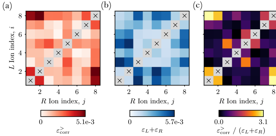
Figure 5.13: Correlated and local error per Cliffords measured for all qubit pairs after applying k -copy RB to an 8 ion chain. Noise is dominated by position dependent duration of R_x(\pi/2) gates consistent with inhomogeneous illumination by the global drive. Panel (a) displays the extracted excess correlated errors, \varepsilon_{\text{corr}}^{(i,j)} for each qubit pair, (i, j) . Panel (b) displays the sum of both independent depolarising errors, (\varepsilon_L + \varepsilon_R)^{(i,j)} . Panel (c) displays the ratio of excess correlated noise to the sum of local errors given in (b). This plot highlights the outer qubits are dominated by spatially correlated errors.
