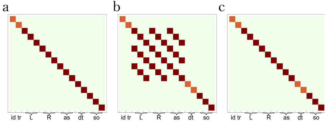
Figure A.1: Liouville operator representation of error channels after twirling over Cl_1^{\otimes 2} , ordered by the Schur basis. (a) Common noise , (b) Continuous ZZ , (c) Stochastic ZZ . Orange blocks represent an entry of 1, green represent 0, and red represent a decay with dependence on m .
