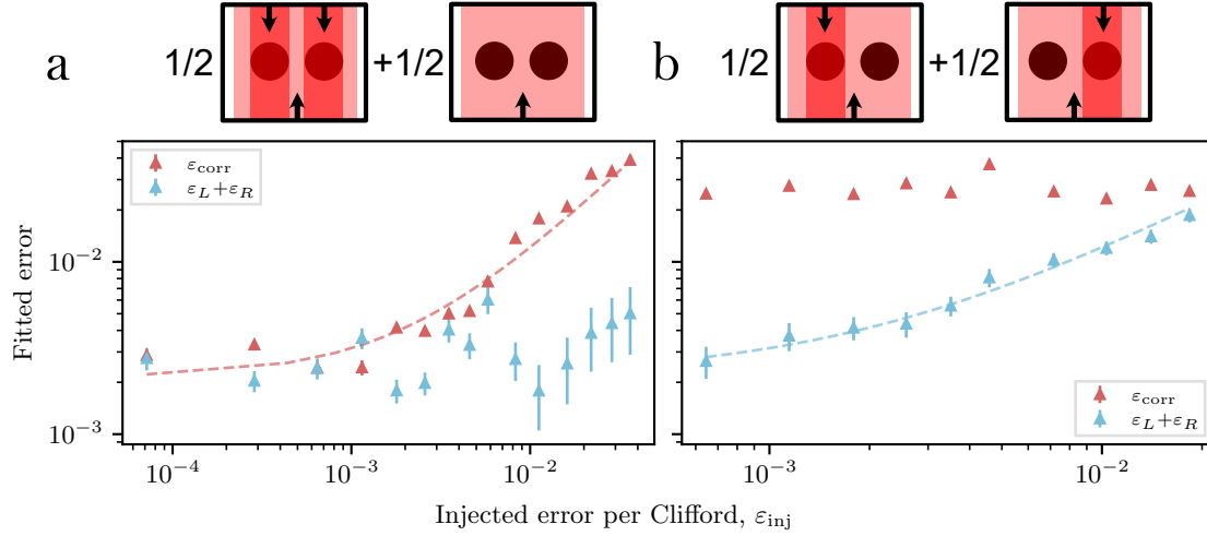
Figure 1.11: Correlated and uncorrelated errors are injected via a single-addressed Stark-shift beam, and quantified through fitting the correlated success populations. The four addressing configurations are depicted visually above the plot. The wide beam signifies the on-resonance global drive which executes the parallel single-qubit rotations, while the narrow beams represent the off-resonant Stark shift beams addressing single-qubits (black circles). In (a) the errors are correlated between qubits, while panel (b) shows the extracted errors after independent errors are injected. Error bars are the extracted standard deviations from a non-linear Levenberg–Marquardt fit of the underlying correlated populations.
