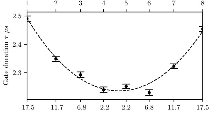
Figure 1.13: Variation of \pi -pulse gate duration along eight ion chain due to global beam Gaussian profile.
