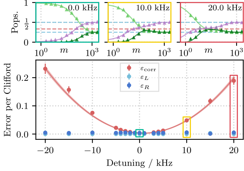
Figure 1.10: Remake figure for thesis. Correlated and single-qubit depolarising errors extracted as a function of shared-drive detuning. The correlated error (red points) rises quadratically with laser detuning, while the local depolarising errors (blue points) remain approximately constant. Error bars are the extracted standard deviations from a non-linear Levenberg–Marquardt fit of the underlying correlated populations. The red shaded region signifies the 68% confidence, generated through covariance-based parameter sampling.
