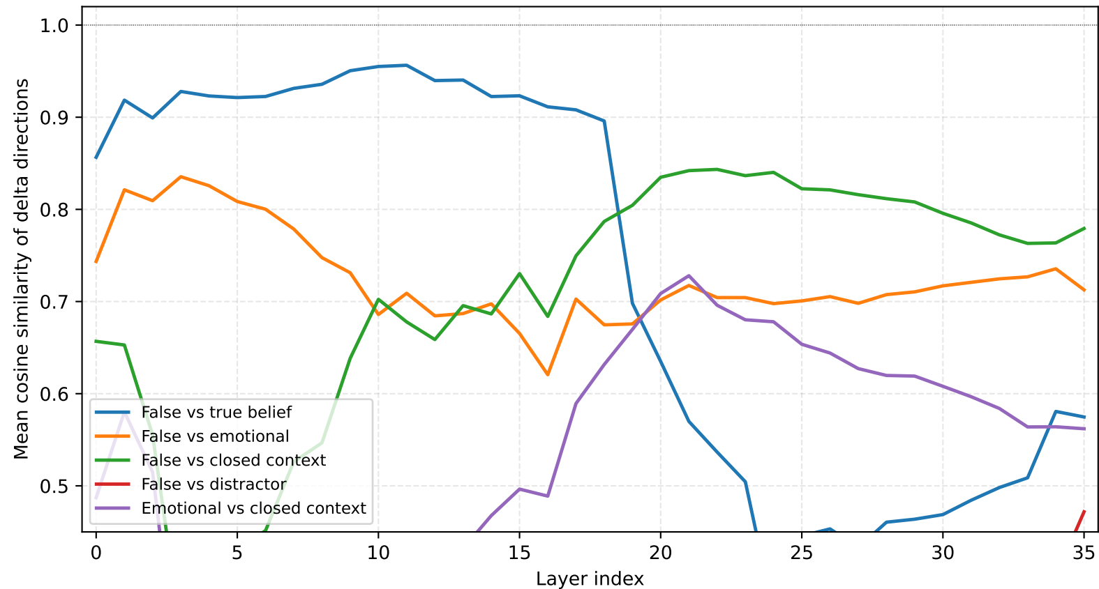
Figure 3. Layerwise cosine similarity between pressure delta directions
