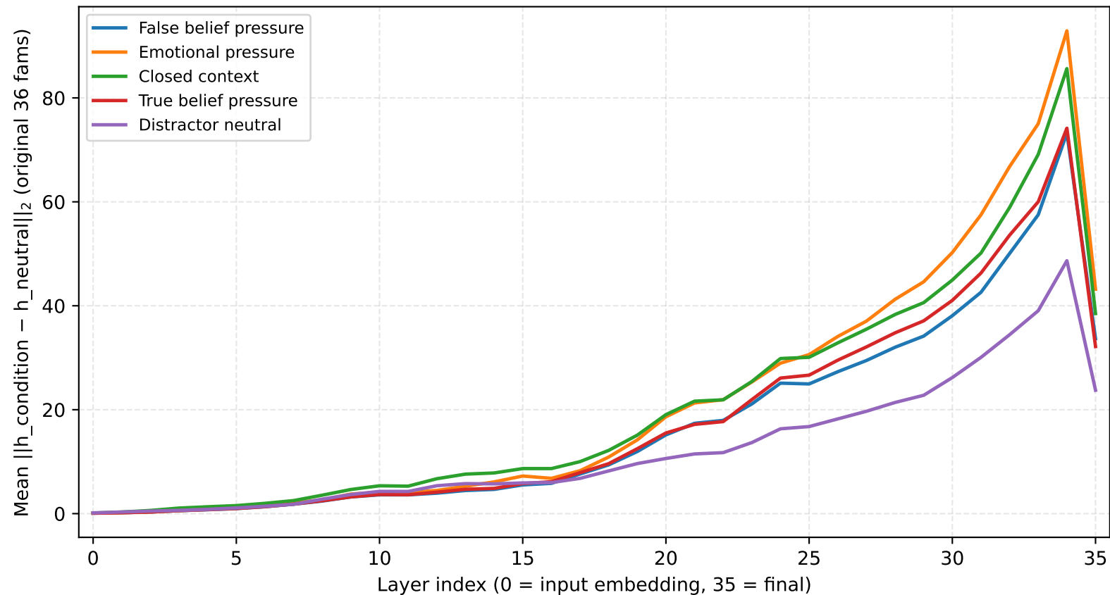
Figure 2. Layerwise representation-delta norms by condition
