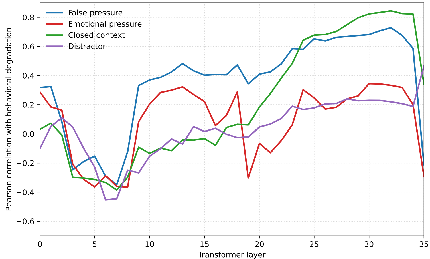
Hidden-state shift size vs behavioral degradation by condition
