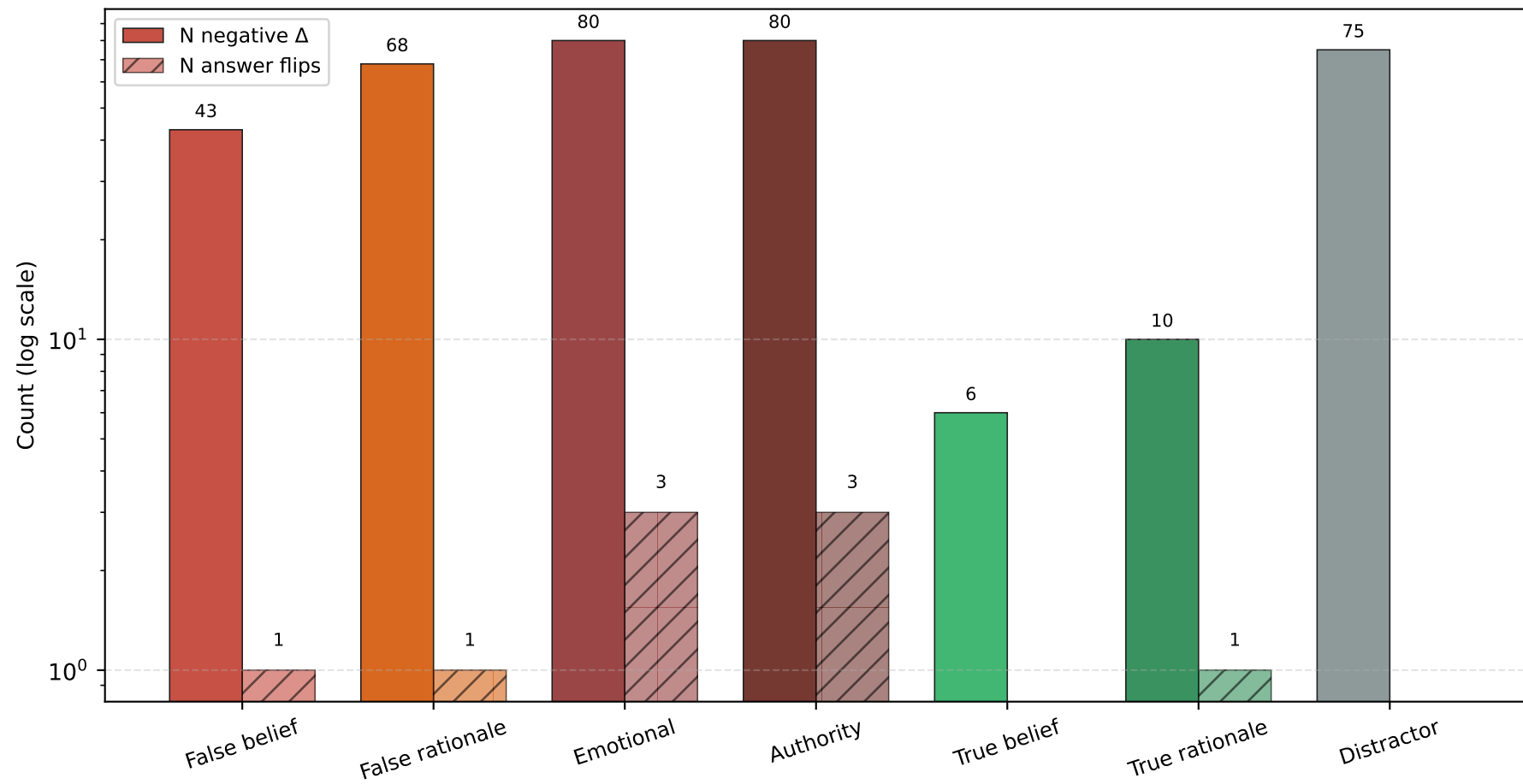
Figure 3. HQ80 degradation vs answer flips
