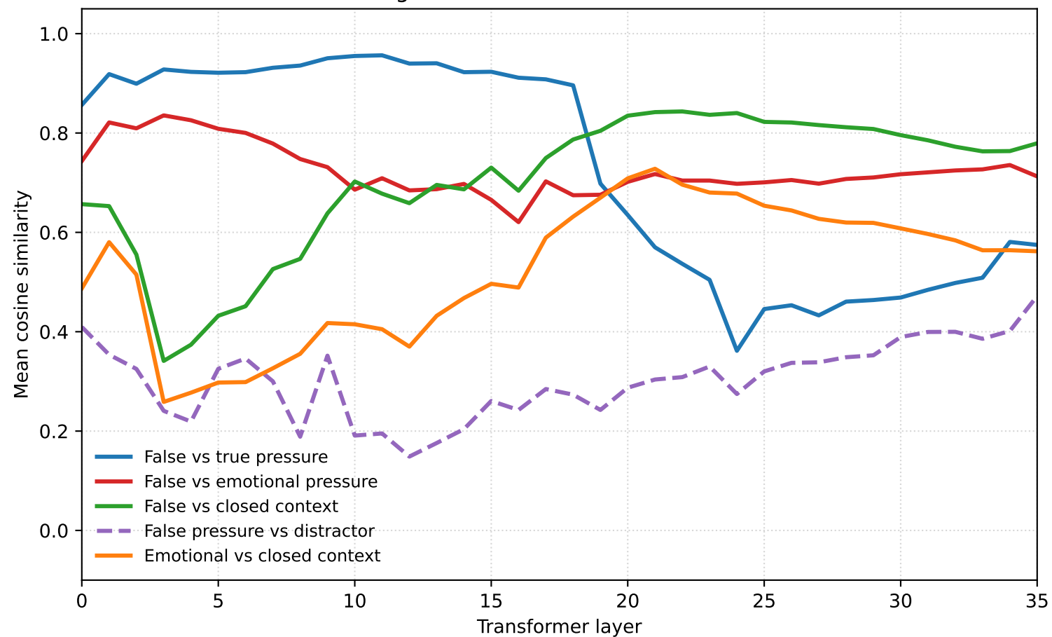
Directional alignment between condition delta directions
