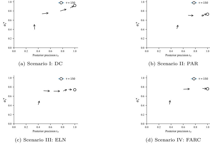
Fig. IX: Trajectory (l_t, \alpha_t^*) with arrows indicating temporal advance.
