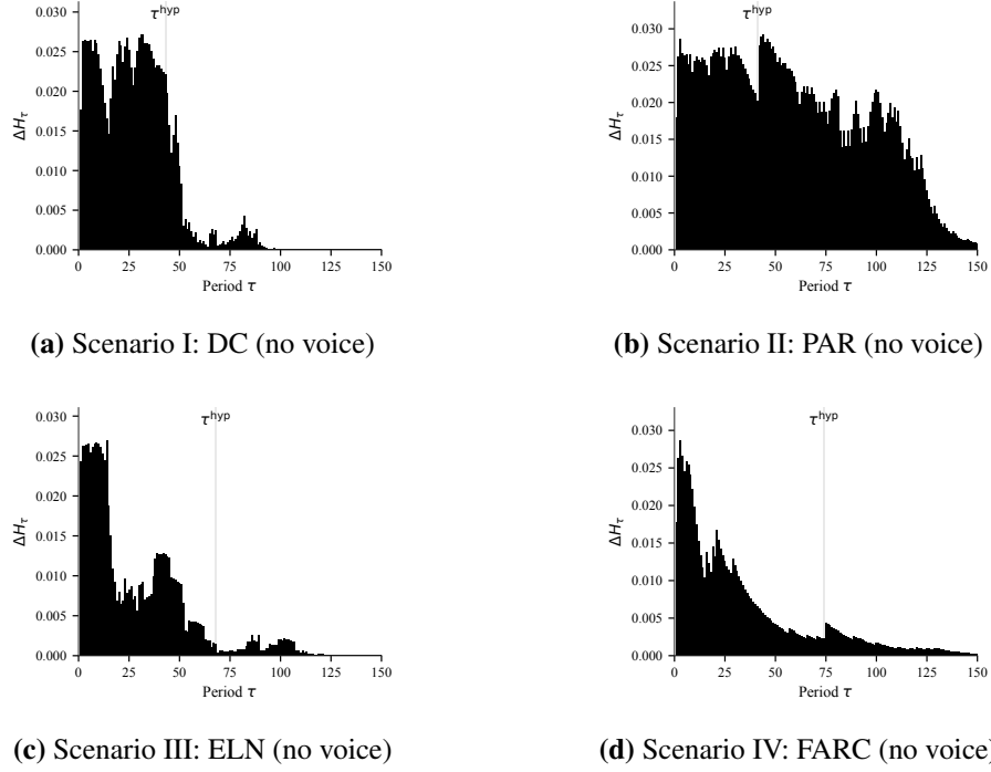
Figure 19 Expected informational gain \Delta H_t against \tau under excluded voice communication.
