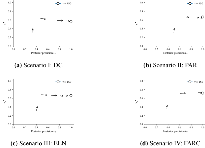
Figure 8 Trajectory (l_t, \gamma_t^*) with arrows indicating temporal advance.
