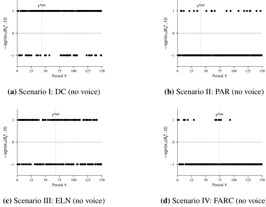
Figure 20 Net sensitivity \kappa_h(\theta_K^*, t) of expected captivity duration with respect to \gamma_t^* under excluded voice communication.
