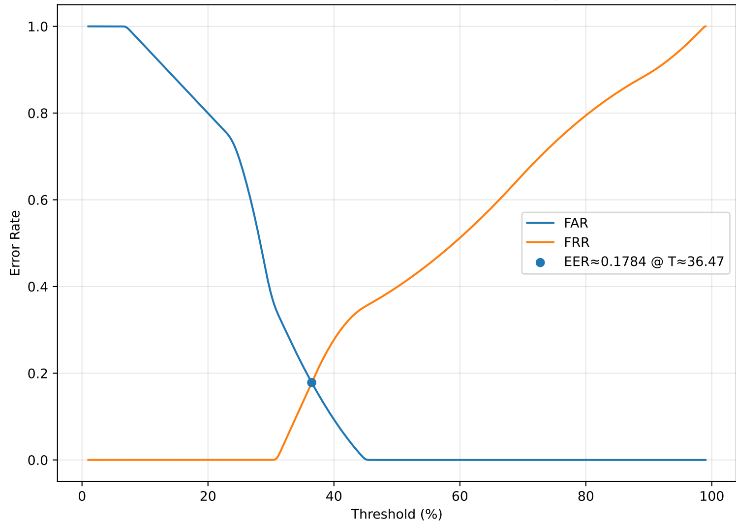
LivDet FAR / FRR vs Threshold (best score over probes)
