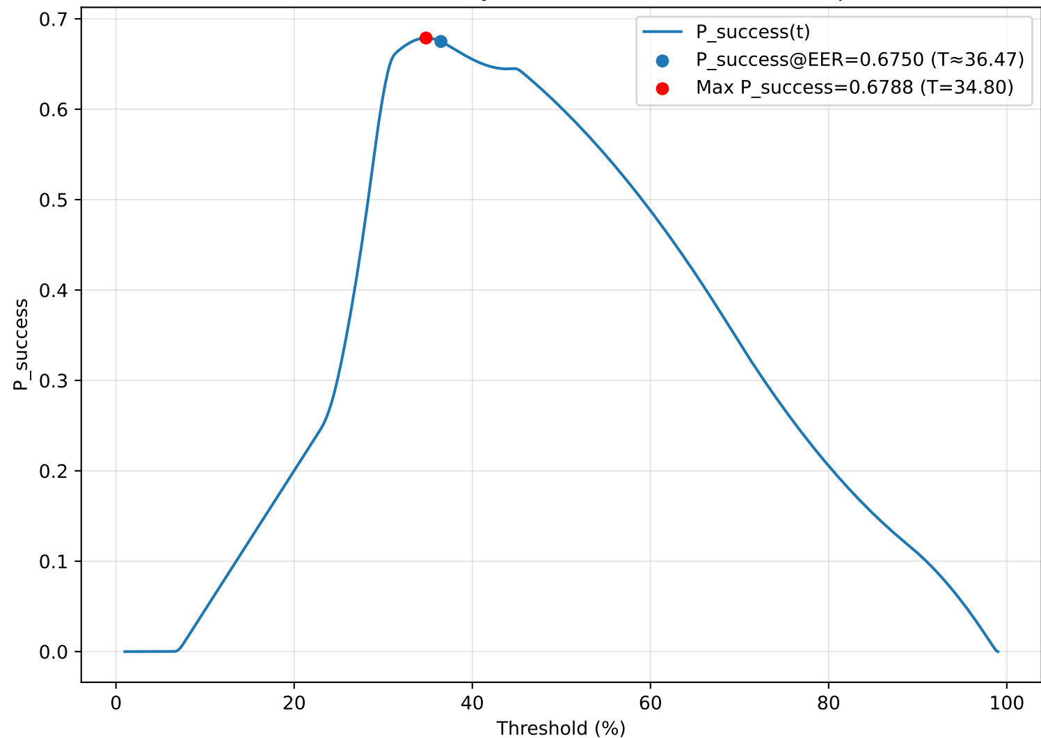
LivDet Success Probability vs Threshold (best score over probes)
