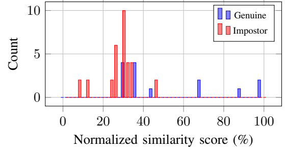
Figure 17: LivDet score histogram using the best score over probe templates.
