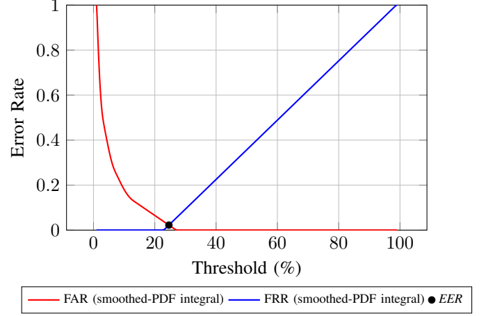
Figure 15: FAR and FRR as a function of the decision threshold, with the Equal Error Rate ( EER ) point.
