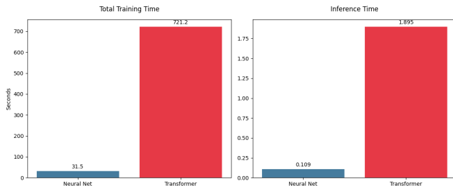
Fig. 7: Total training time (left) and inference latency (right) comparison, highlighting the high cost of attention mechanisms.
