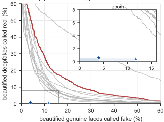
(a) FF++ c23 test, paired beautification
