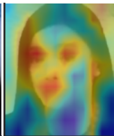
evidence -> filter (0.86)
