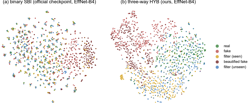
Fig. S6. t-SNE of penultimate features on the same FF++ test images (300 per group). (a) The official SBI checkpoint separates forgeries, but beautified genuine faces are mixed with real faces, as a binary label space requires. (b) HYB forms a filter region, and beautified forgeries stay in the fake region. Of the ten nearest labelled neighbours of a beautified forgery, 11.7% are genuine for SBI and 4.2% for HYB.
