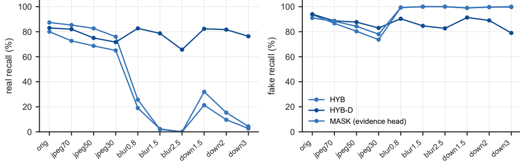
Fig. S8. Recall of genuine (left) and forged (right) FF++ test frames under JPEG re-compression, Gaussian blur and downscaling (300 frames each). Models trained without symmetric degradation call almost every blurred genuine frame fake.
