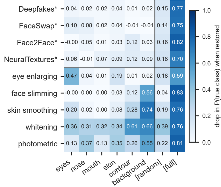
Fig. S7. Region restoration on correctly classified FF++ test images: drop in P(\text{true class}) when one facial region is restored to its unedited pixels. [random]: area-matched patch at a random location; [full]: whole image restored. *Forgeries use the real frame of the same video, resized to the fake crop (approximate alignment).
