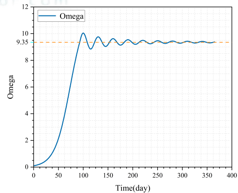
(b) Maturity Index of Ecosystem
