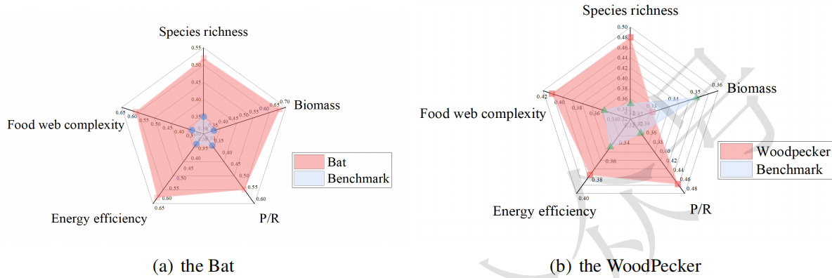
Figure 12: Woodpeckers and Bats
