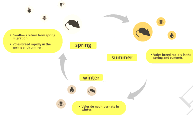
Figure 6: Seasonal Ecosystem of North Temperate Wheat Fields
