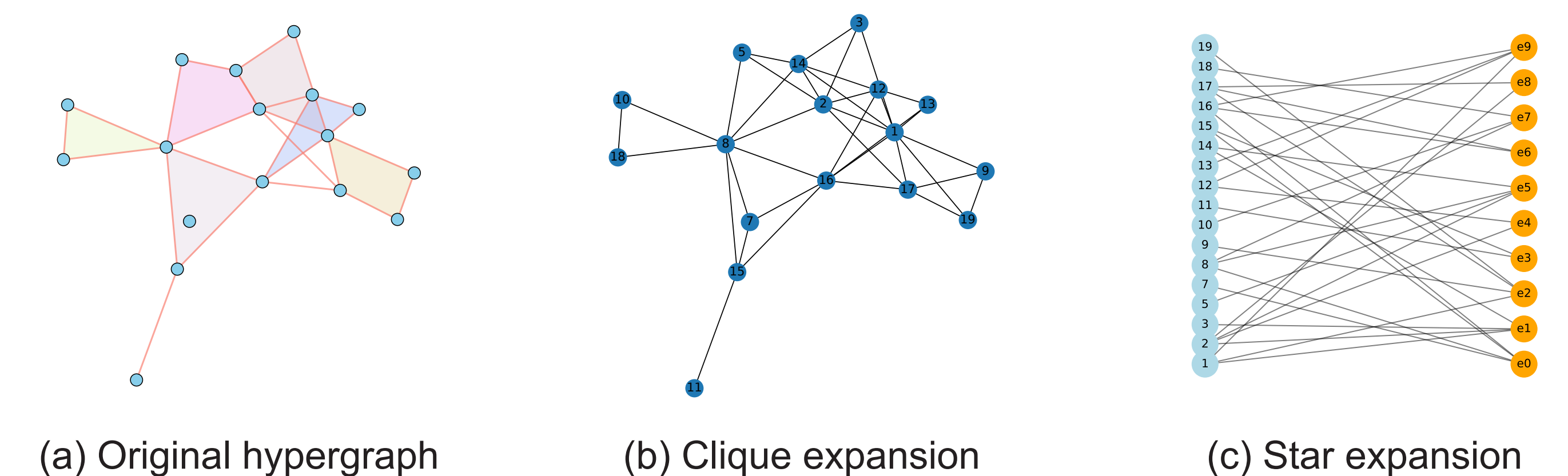
A hypergraph and its clique and star expansions
