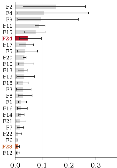
ResNet
