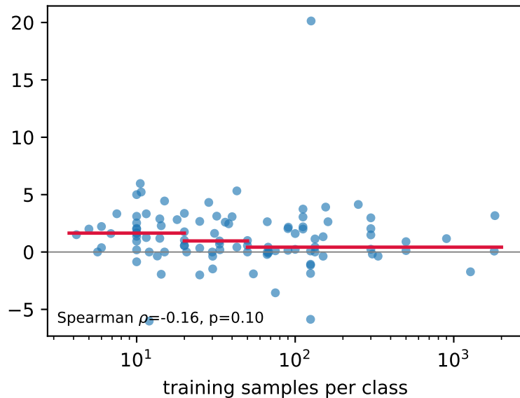
ResNet
