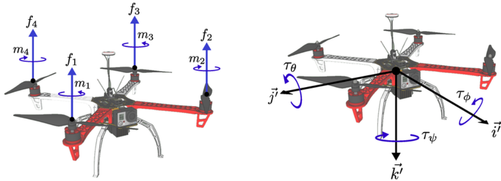
Figure 1: typical quadcopter setup 'props-in', yaw \psi (turning around), pitch \theta (nose up or down) and roll \phi (tilting to sides) From [?] ]
