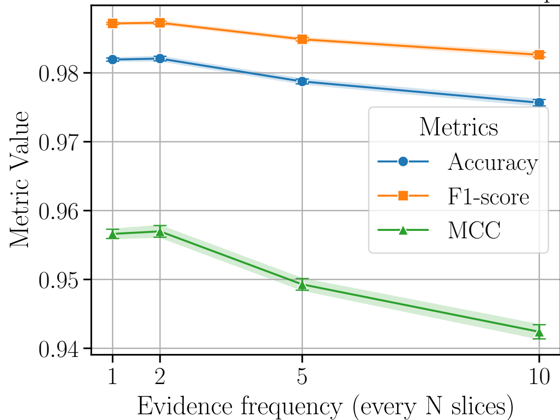
5-fold Cross-Validation Metrics vs evidence frequency
