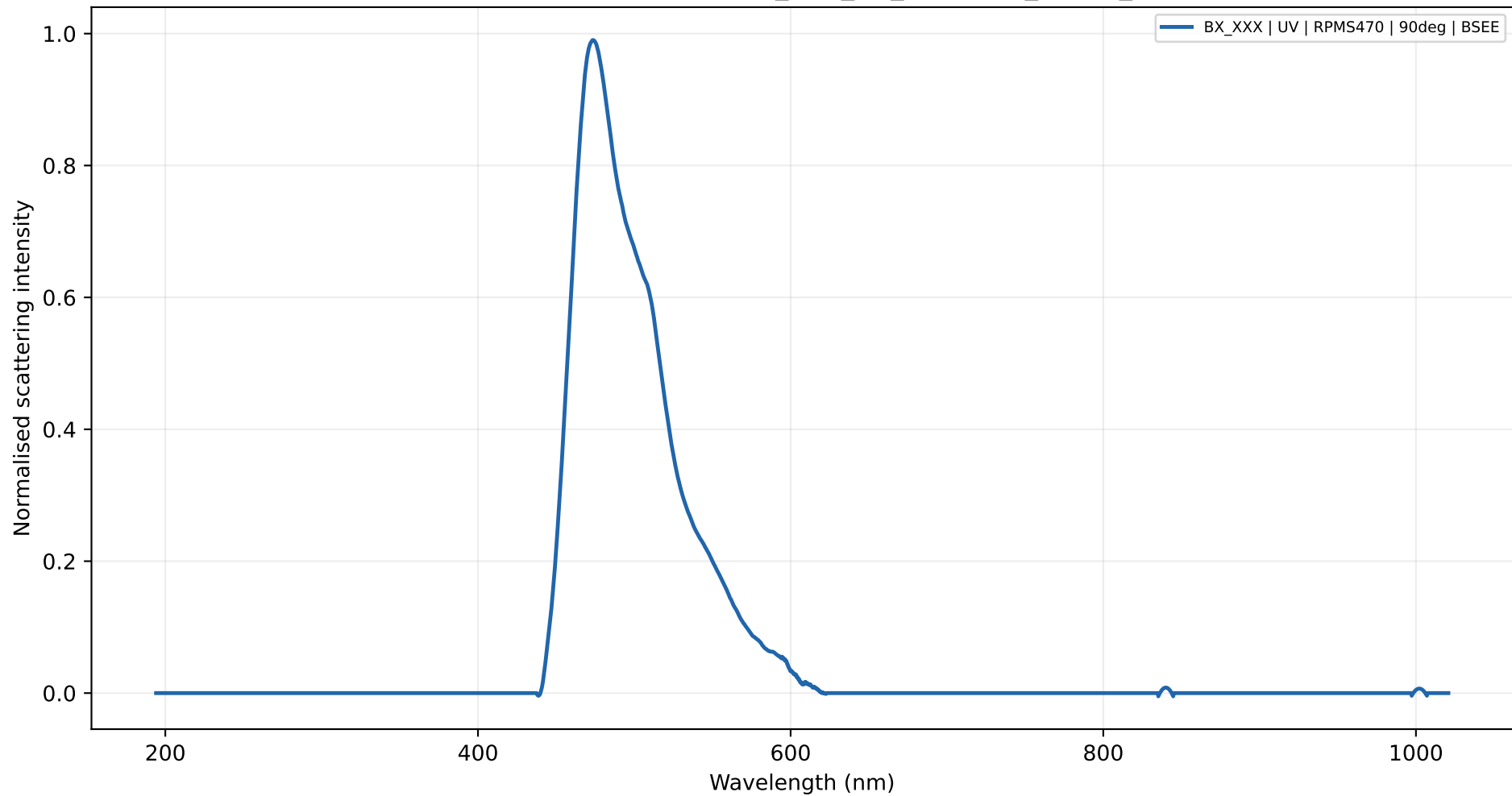
Scattering shape 90deg - BX_XXX_UV_RPMS470_90deg_BSEE
