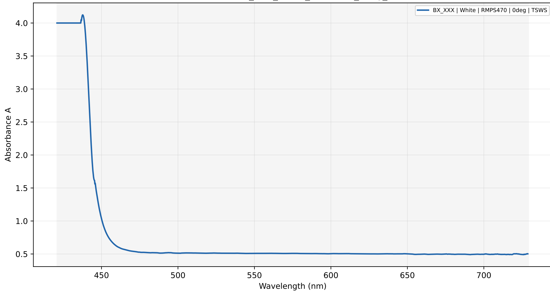
Absorbance - BX_XXX_White_RMPS470_0deg_TSWs
