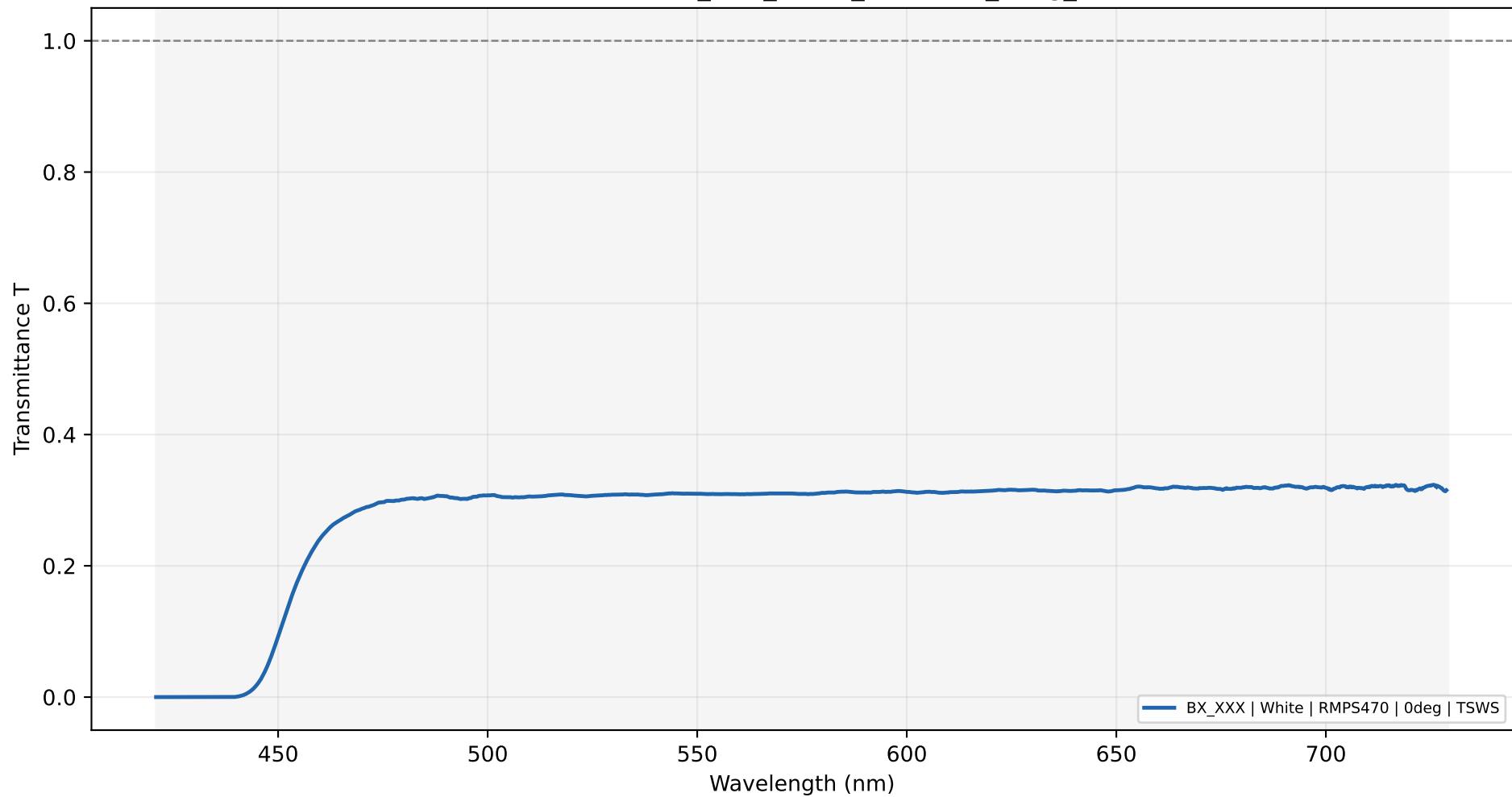
Transmittance - BX_XXX_White_RMPS470_0deg_TSWs
