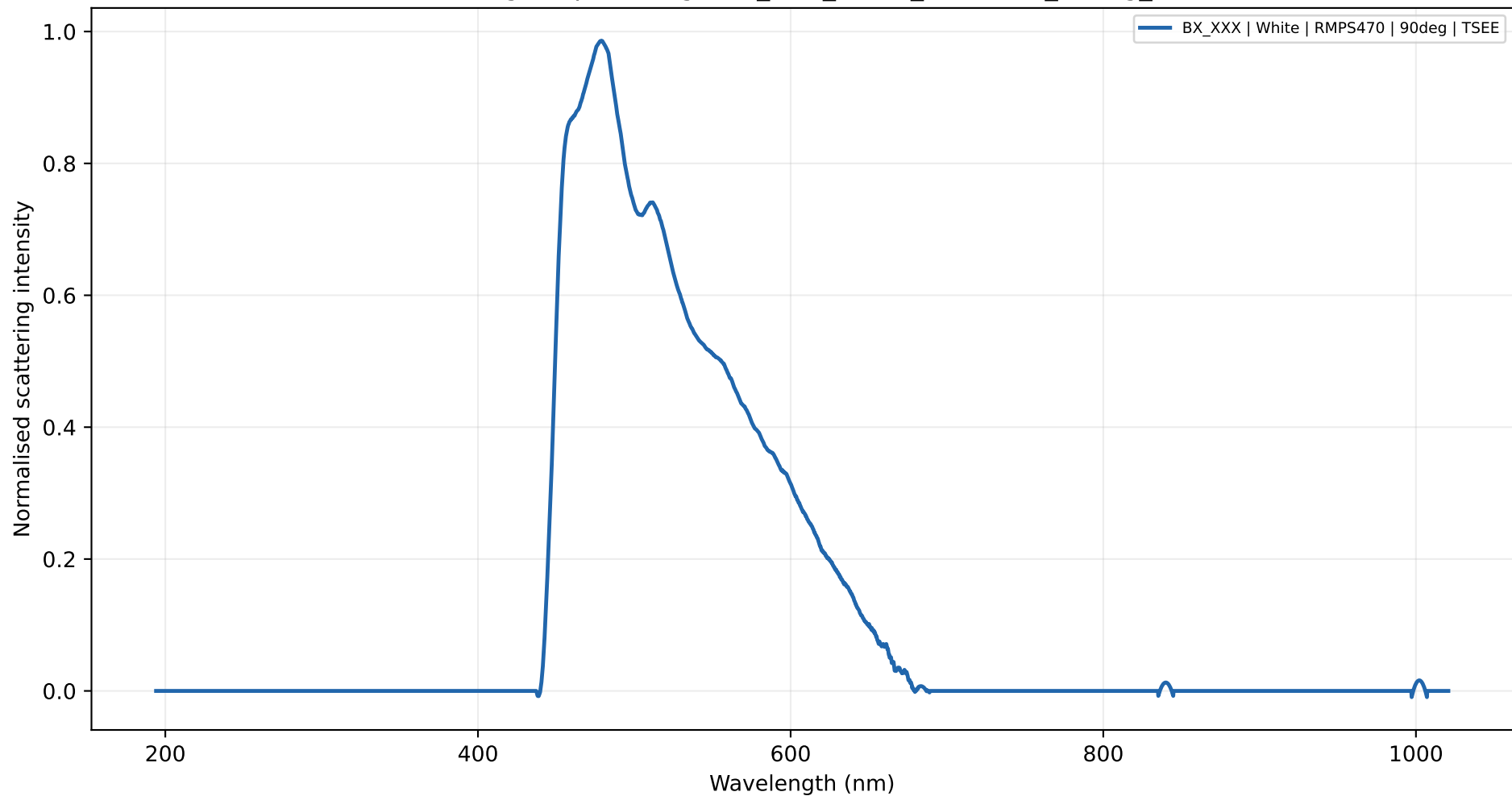
Scattering shape 90deg - BX_XXX_White_RMPS470_90deg_TSEE
