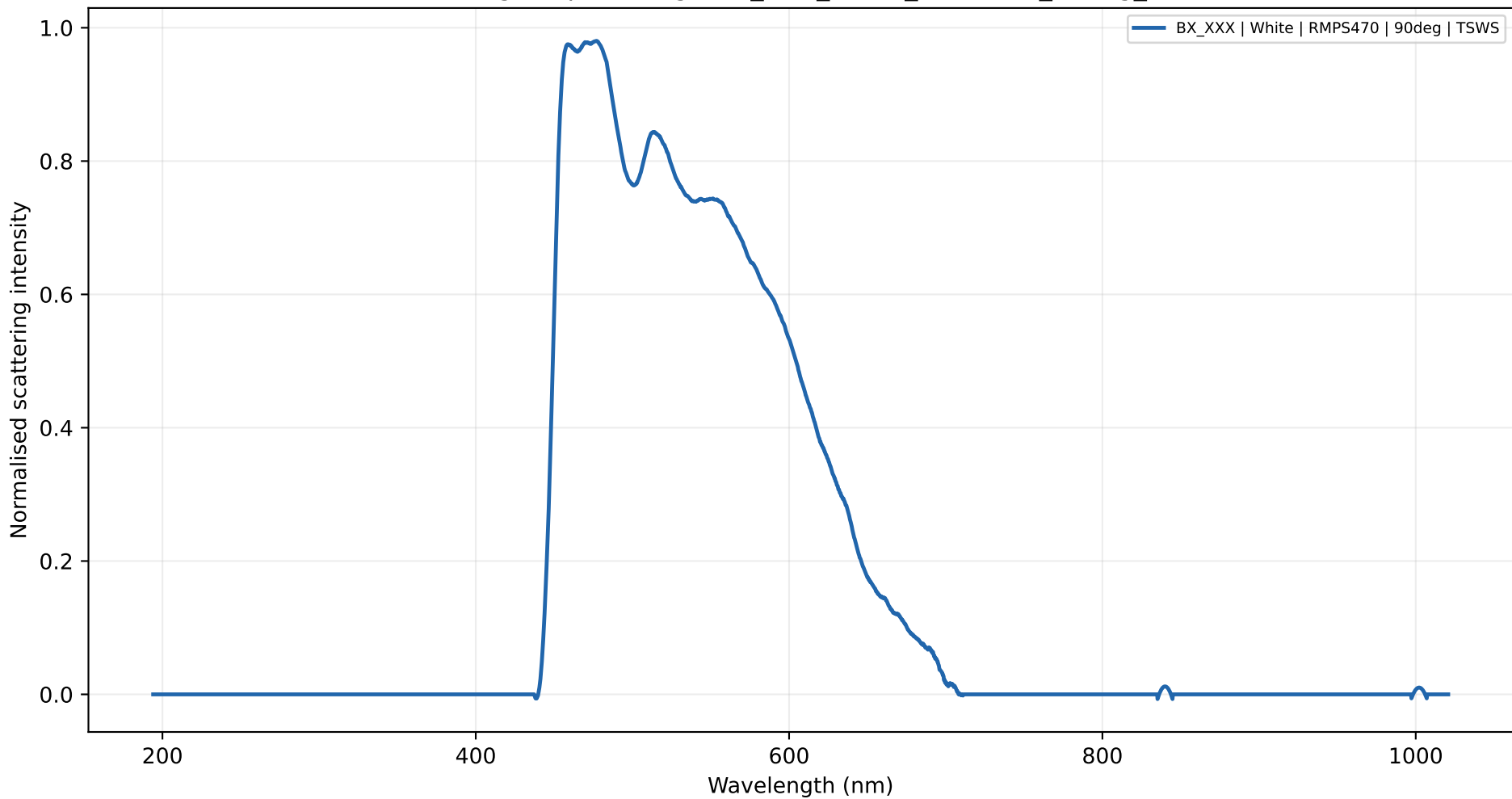
Scattering shape 90deg - BX_XXX_White_RMPS470_90deg_TSWs
