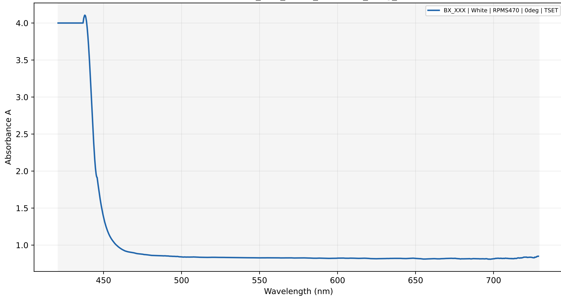
Absorbance - BX_XXX_White_RPMS470_0deg_TSET
