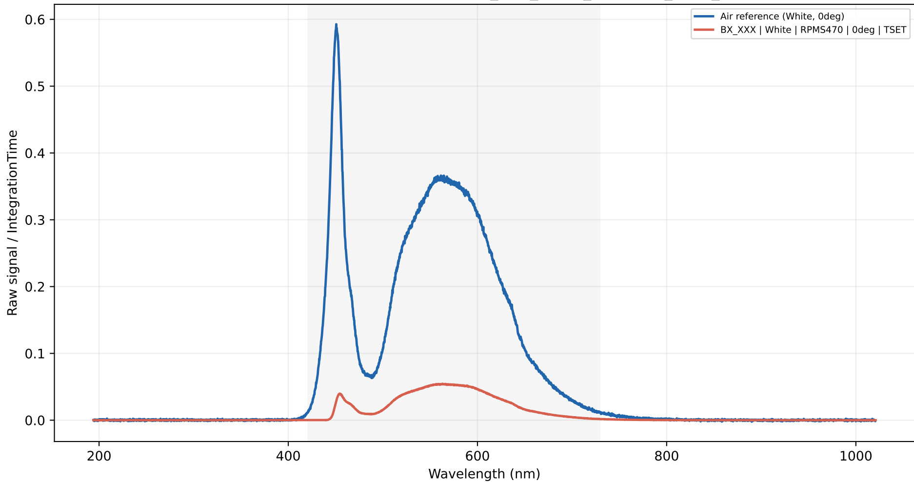
Raw measurement comparison - BX_XXX_White_RPMS470_0deg_TSET
