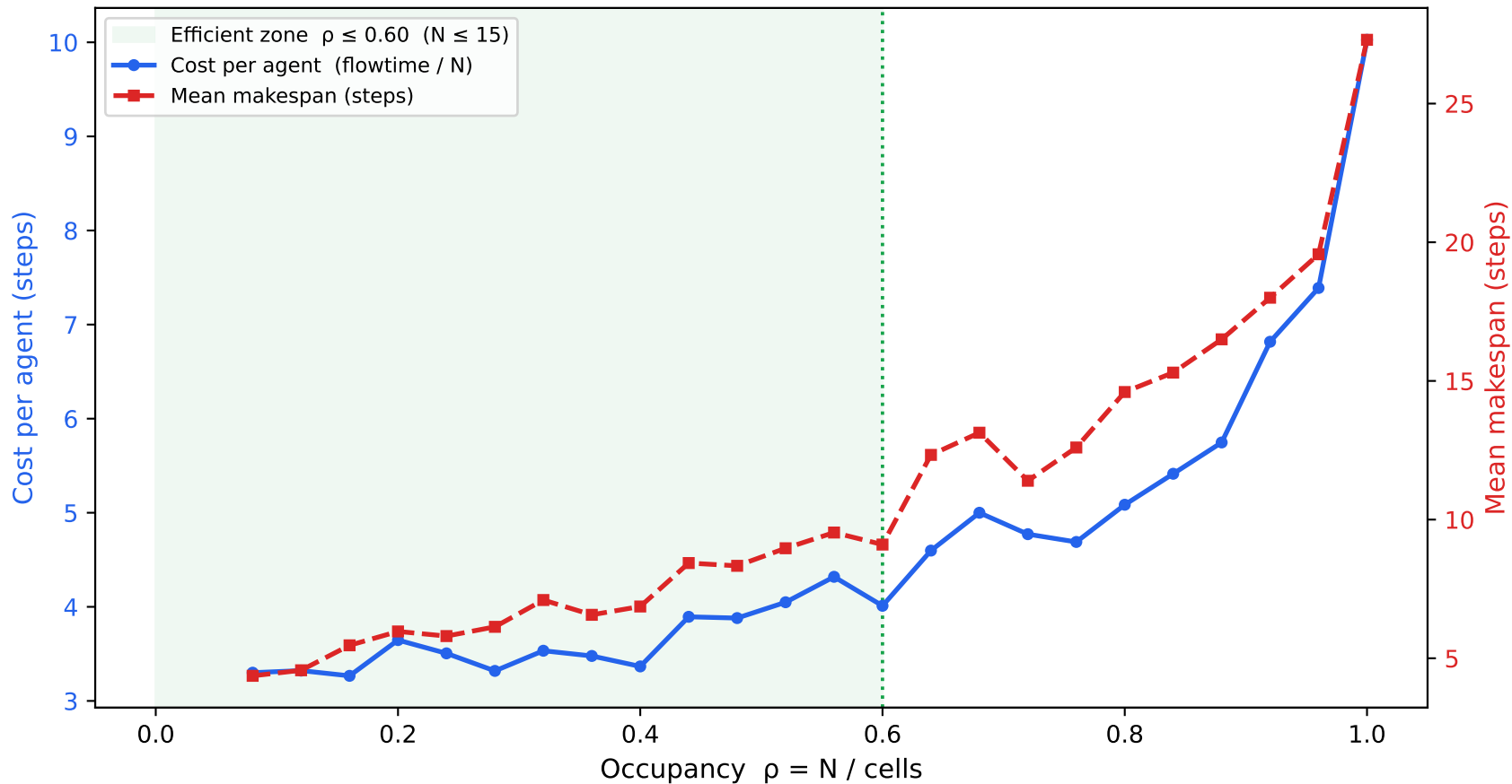
Cost per agent and mean makespan vs. occupancy \rho — both metrics accelerate past \rho = 0.6 (5×5 grid, 400 mm cells, 30 seeds)
