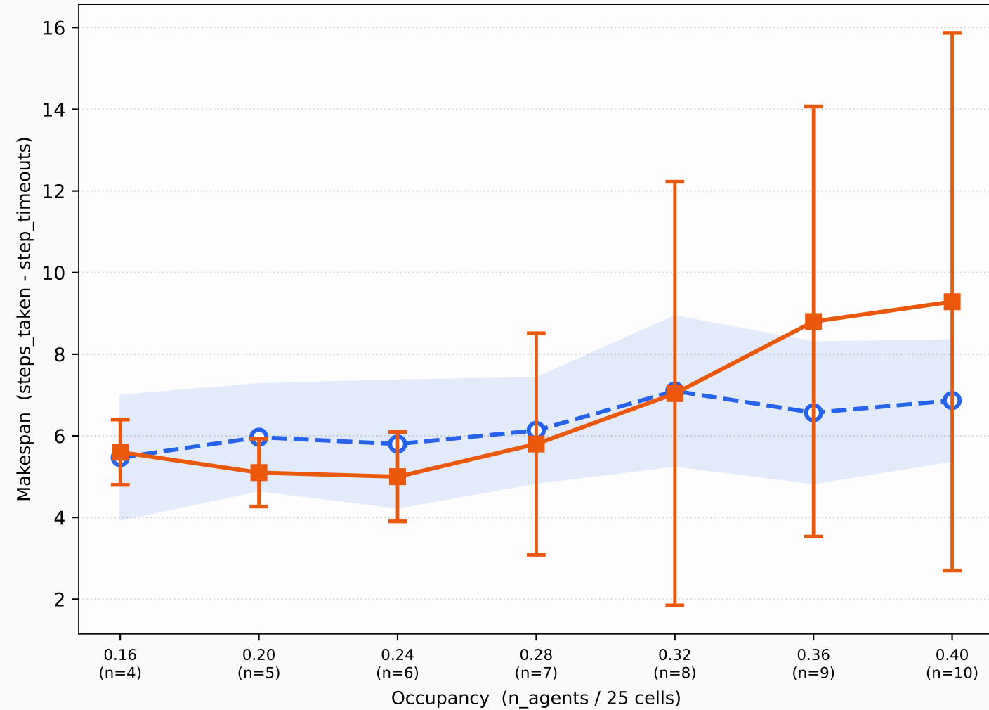
Makespan vs. Occupancy (5x5 grid, 400 mm/cell)
