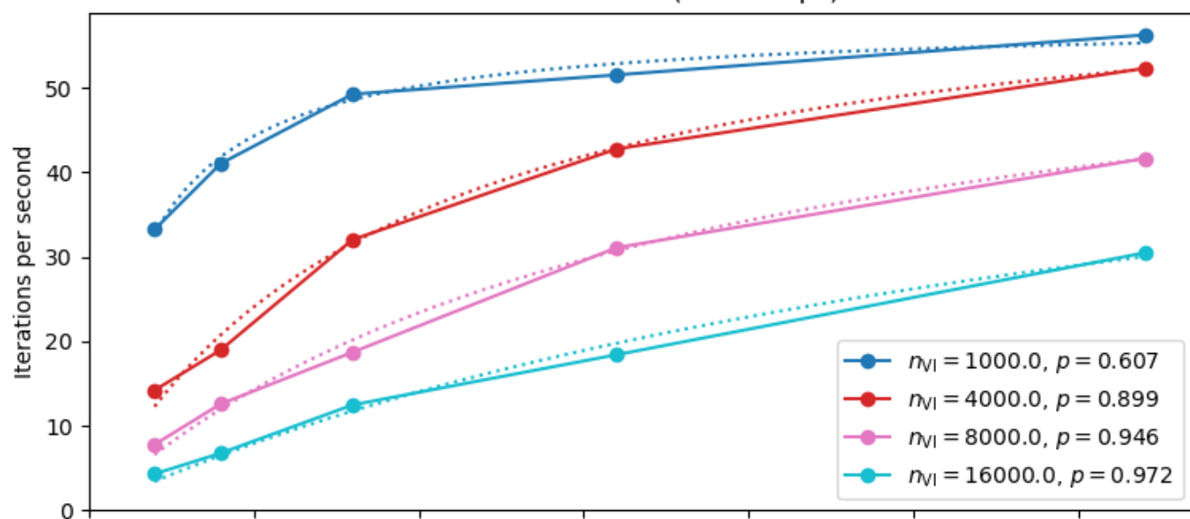
HMC Performance Comparison
