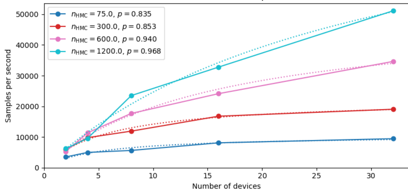
HMC Performance Comparison
