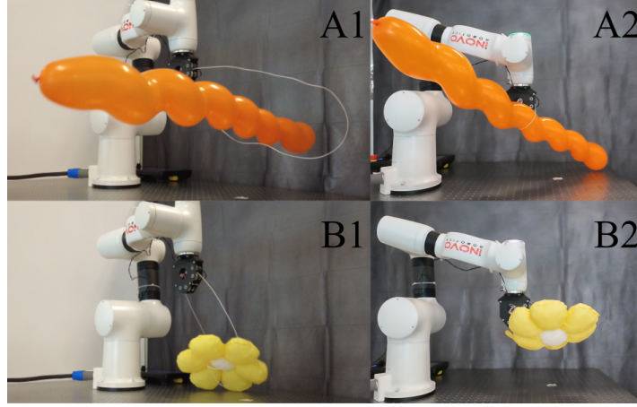
Figure 3.13: Flying object is captured by Lasso Gripper.
