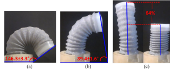
Figure 2.3: flexible fluidic actuators formed with granular to vary stiffness [23]
