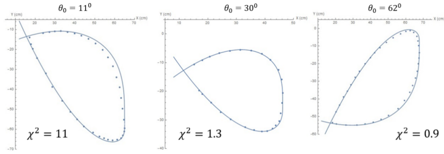
Figure 3.7: The string loop curve fitting of numerical theoretical solution with experimental profiles [1]. In this case, the linear mass \mu = 0.283 \pm 0.005 \text{ g} \cdot \text{m}^{-1} , the length of the string loop L = 160 \text{ cm} , shooting velocity v = 5.1 \text{ m} \cdot \text{s}^{-1} and several values of ejection pitch angle \theta_0 . A satisfactory fitting result with \chi^2 \leq 11 is obtained.
