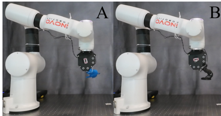
Figure 3.10: Validation of grasping ability via bull and horse figures.
