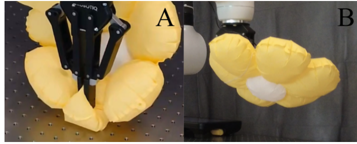
Figure 3.14: The inflated balloon is captured by the antipodal gripper. As a result of the concentrated stress applied, the balloon was severely deformed.
