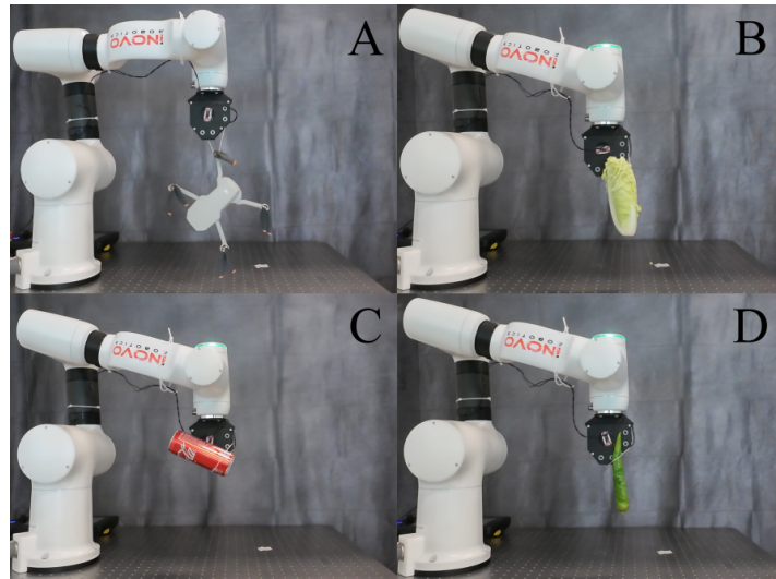
Figure 3.11: Validation of grasping ability over variable shapes: drone, cabbage, coke can and chili pepper.
