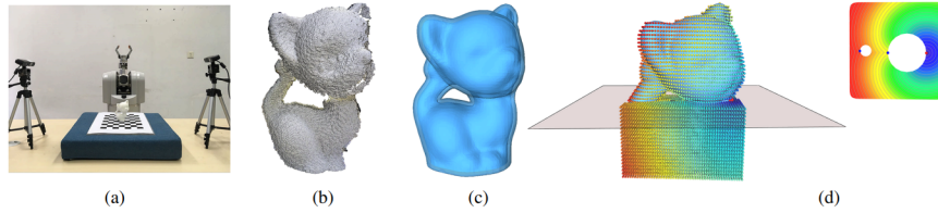
Figure 3.5: The caging loop calculating algorithm for Lasso Gripper [19]. (a) The setup of the depth reconstruction system (b) The Point cloud captured by depth camera directly. (c) A r-offset surface is built for defining the grasping space. (d) Two Morse saddle points (blue) are calculated to define the grasping loop.
