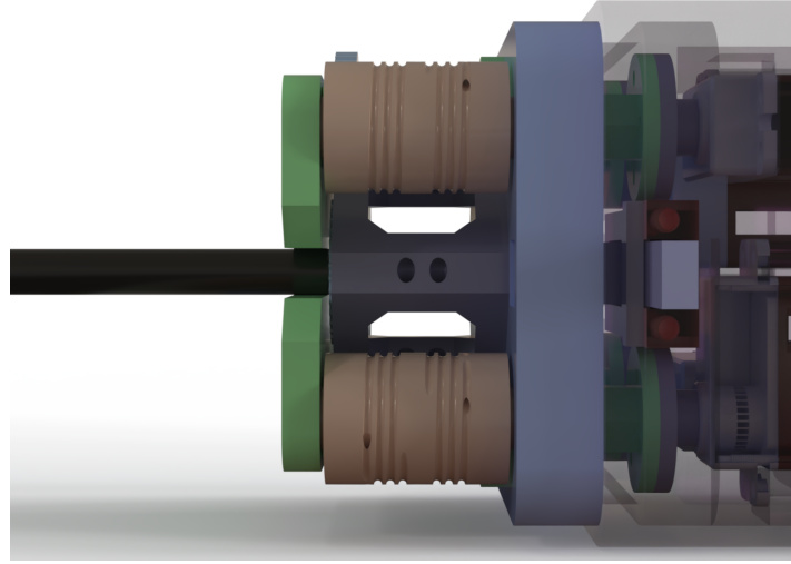
Figure 4.4: Reel Design and Winding Mechanism
